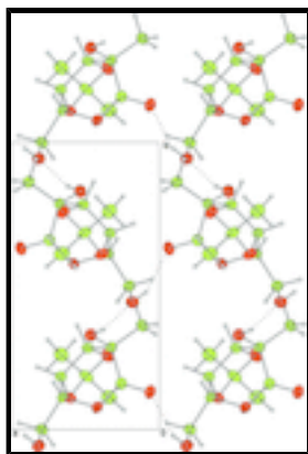
Fig. 4. Packing diagram of the title compound projected along the c -axis. Hydrogen bonds are shown by dotted lines.
