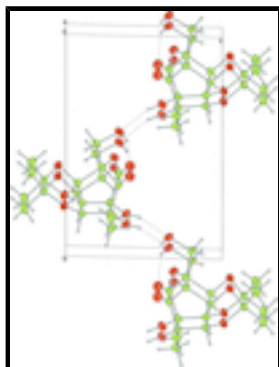
Fig. 3. Packing diagram of the title compound projected along the a -axis. Hydrogen bonds are shown by dotted lines.
